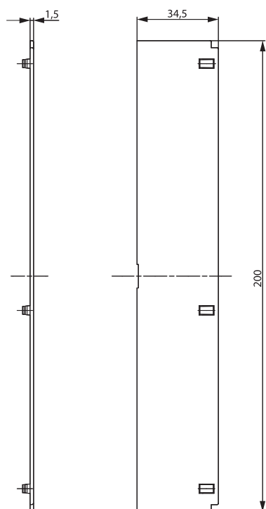
CL-PTV-B D/195
