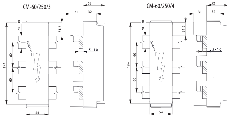
CM-60/250/3/120-5/10
