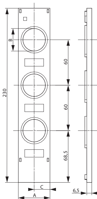
CL-PTV-B D/230
