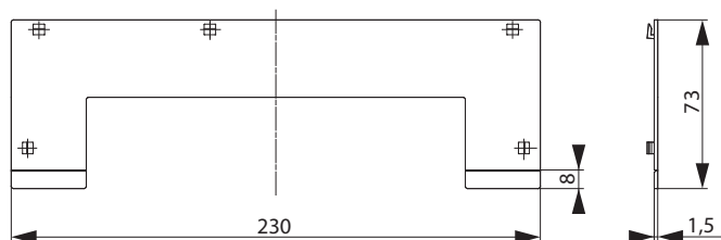
CL-PTV-B D/230
