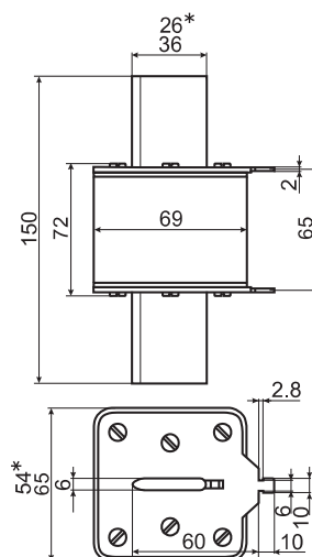
NV/NH 3/3C*
