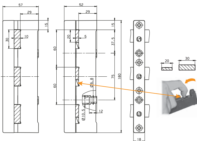
BBS-60/4
