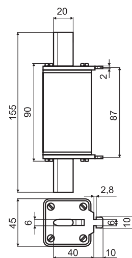
NV/NH 1/1000V
