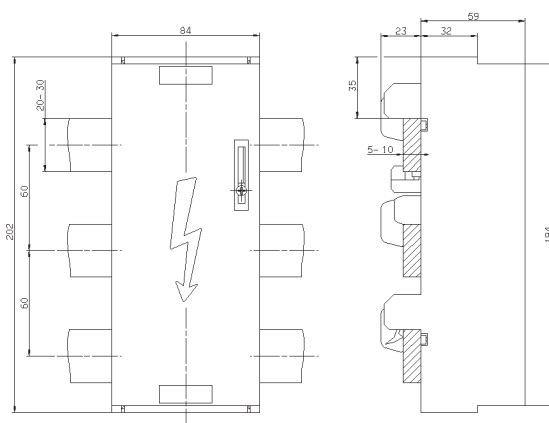
CM-60/250/3/120-5/10
