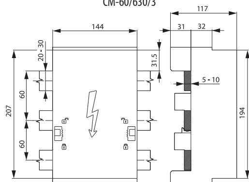
СМ-60/630/3
