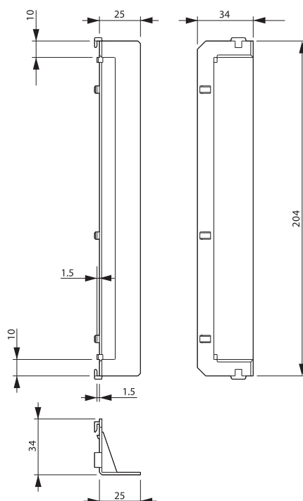
RTP-RL/230
