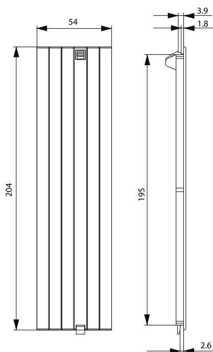
RPH-195
